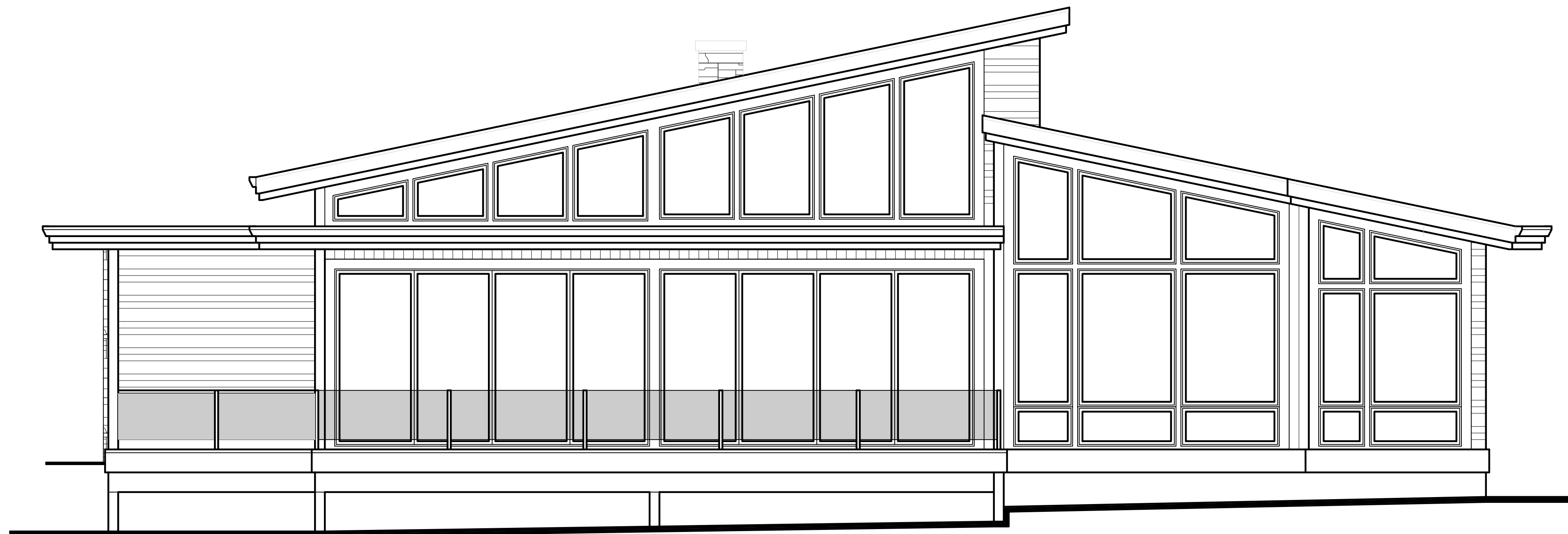
REAR ELEVATION
