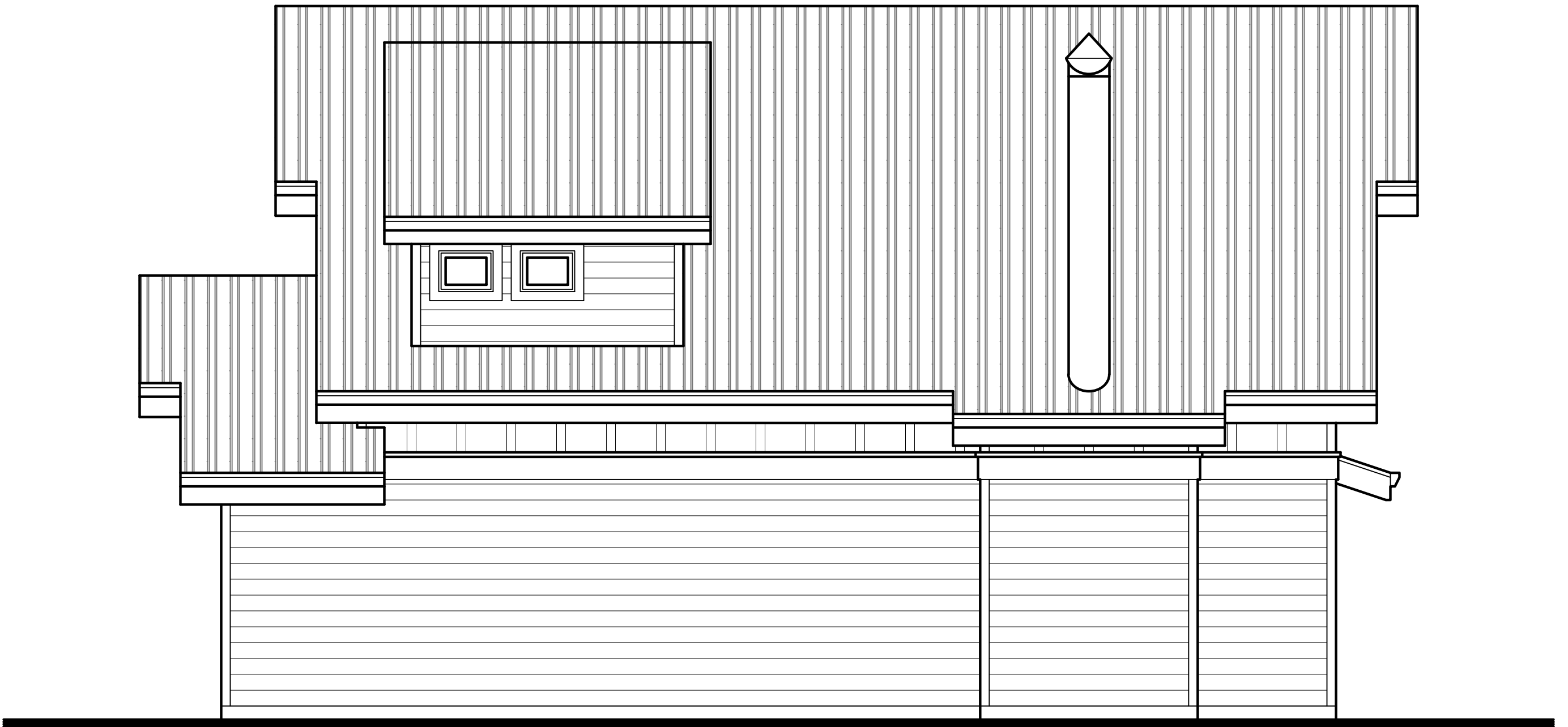
LEFT ELEVATION
