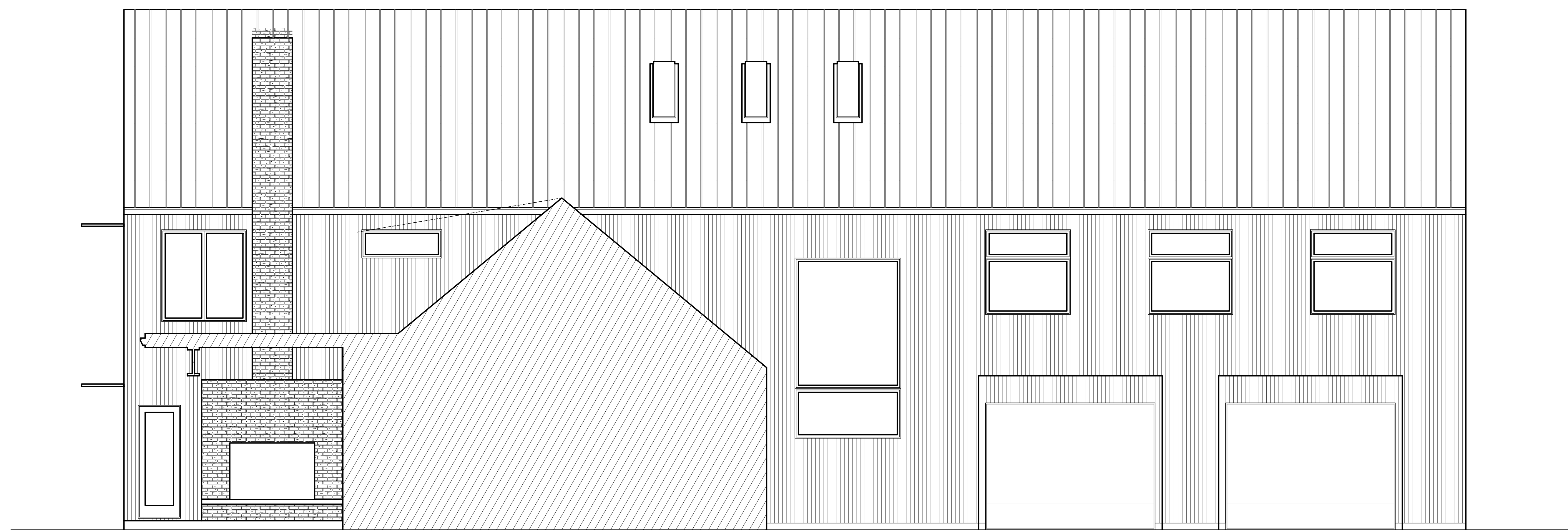
MOTOR COURT LEFT ELEVATION
