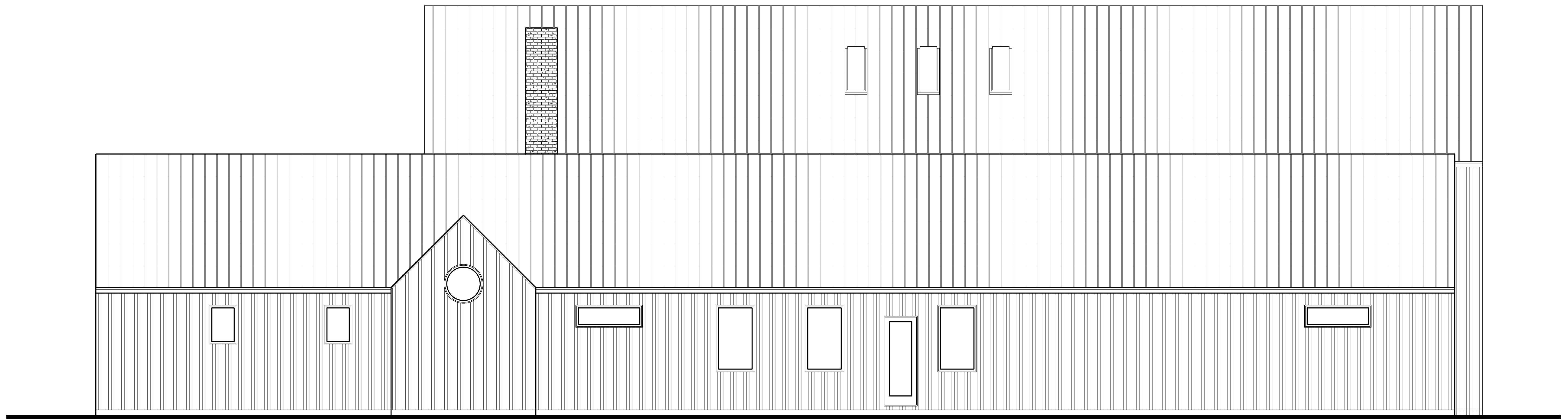
LEFT ELEVATION
