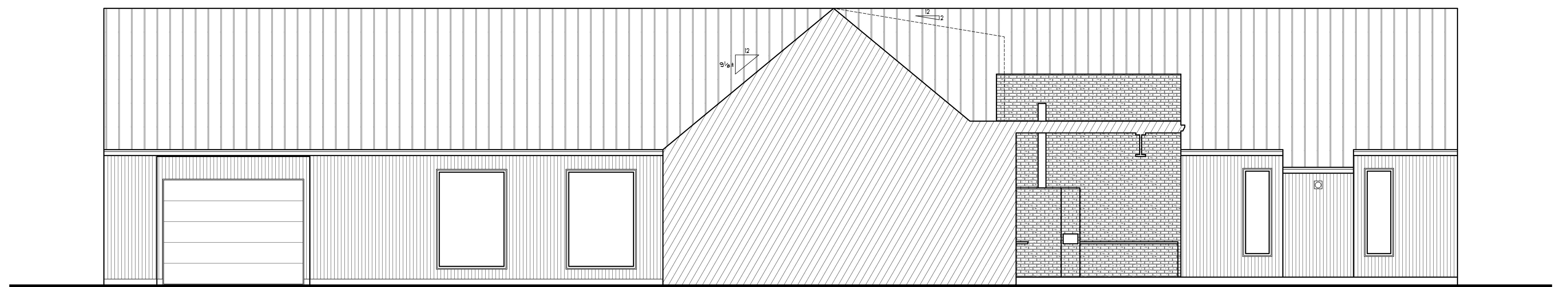
MOTOR COURT RIGHT ELEVATION
