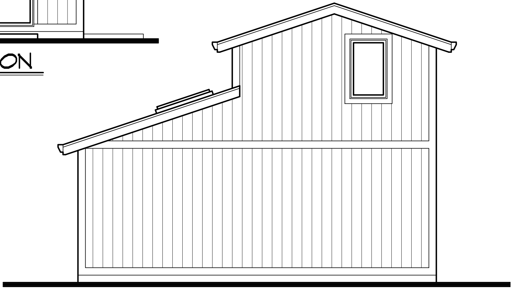
EAST ELEVATION
