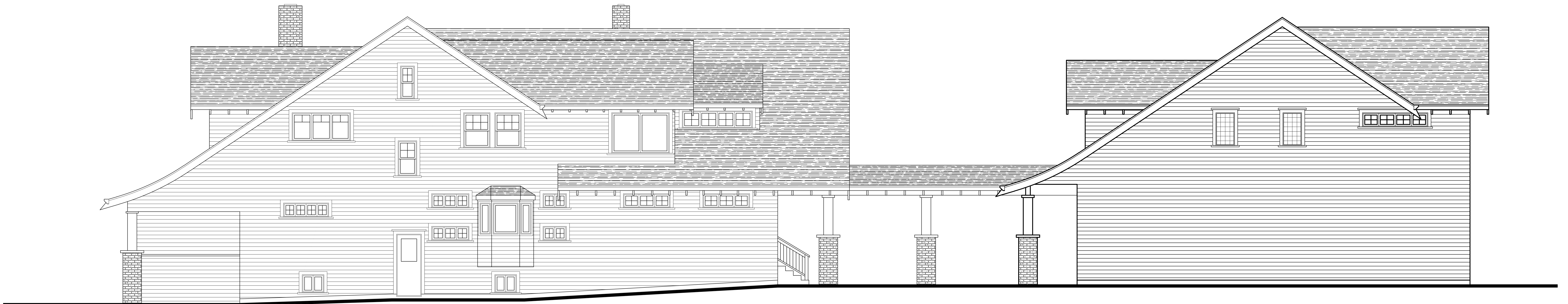
RIGHT SIDE ELEVATION
