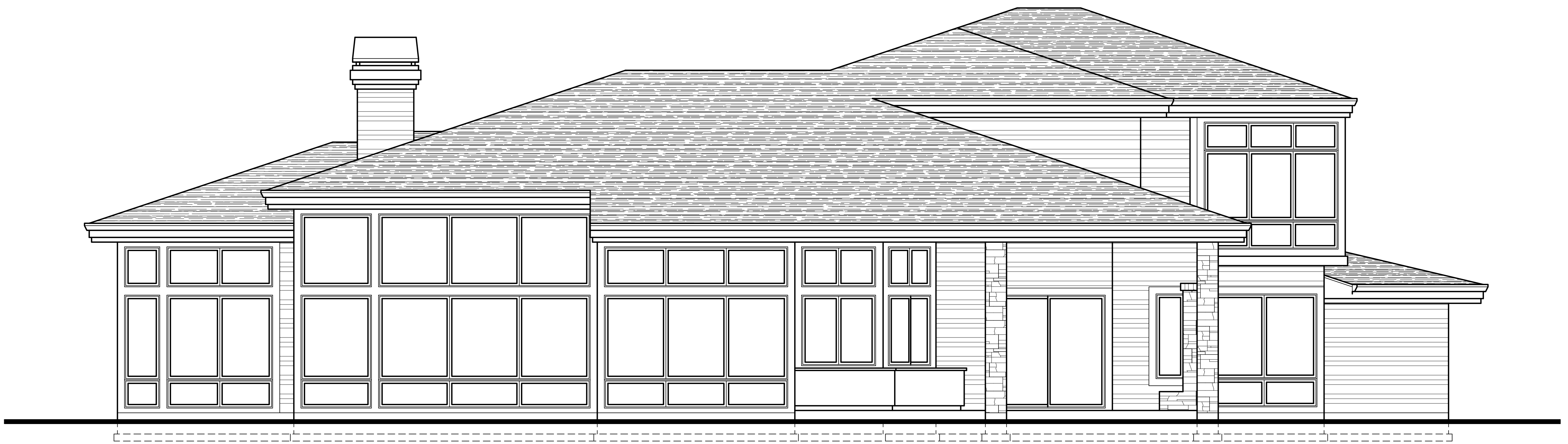
REAR ELEVATION
