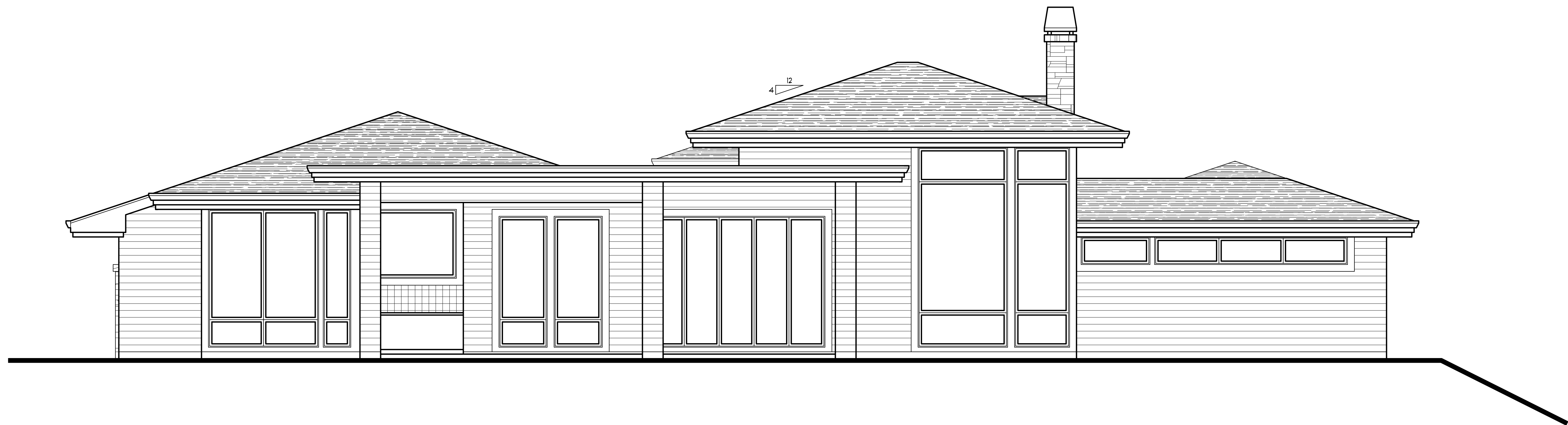
REAR ELEVATION
